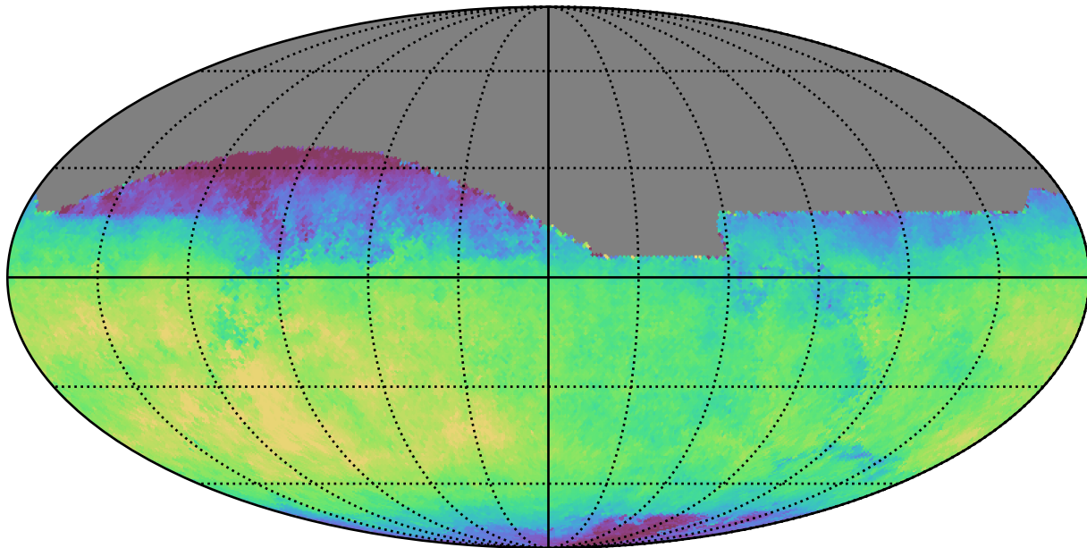
baseline_v3.0_10yrs All sky i band: Median fiveSigmaDepth
