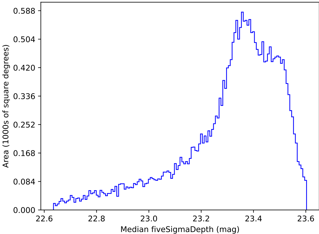
baseline_v3.0_10yrs All sky i band: Median fiveSigmaDepth
