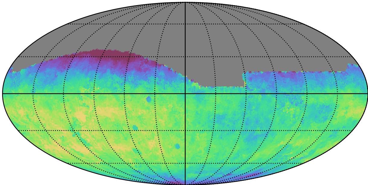
baseline_v3.0_10yrs All sky g band: Median fiveSigmaDepth
