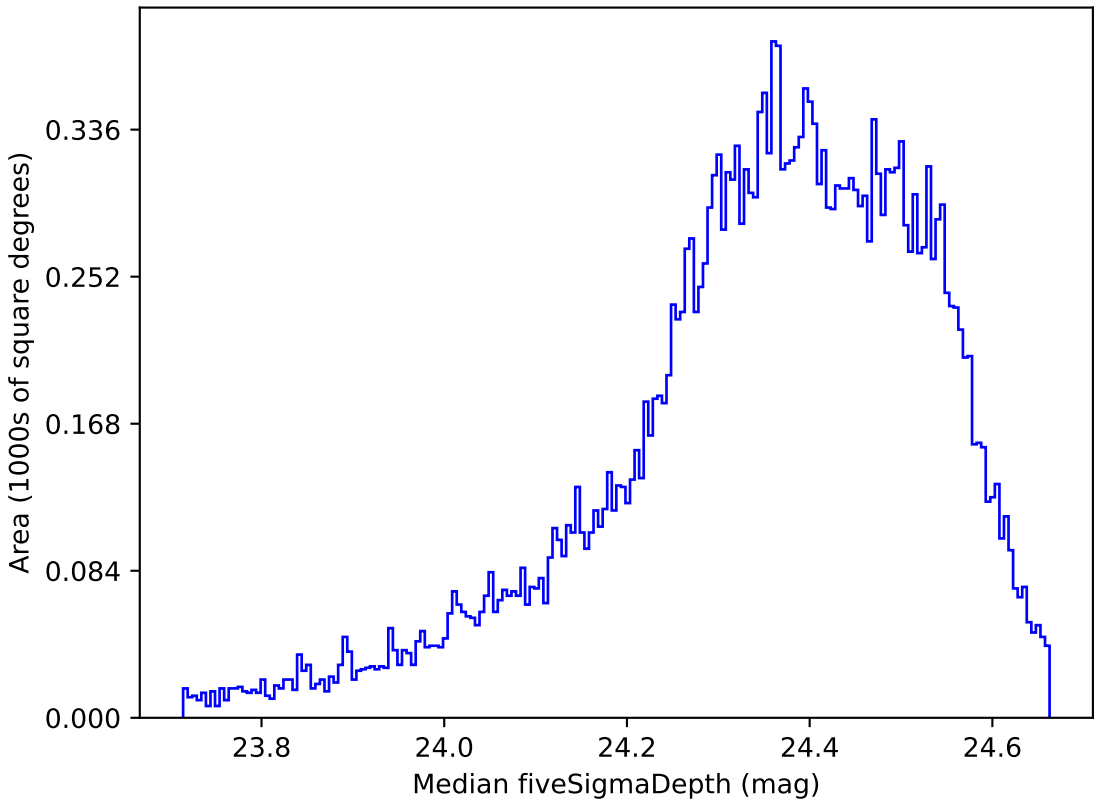
baseline_v3.0_10yrs All sky g band: Median fiveSigmaDepth
