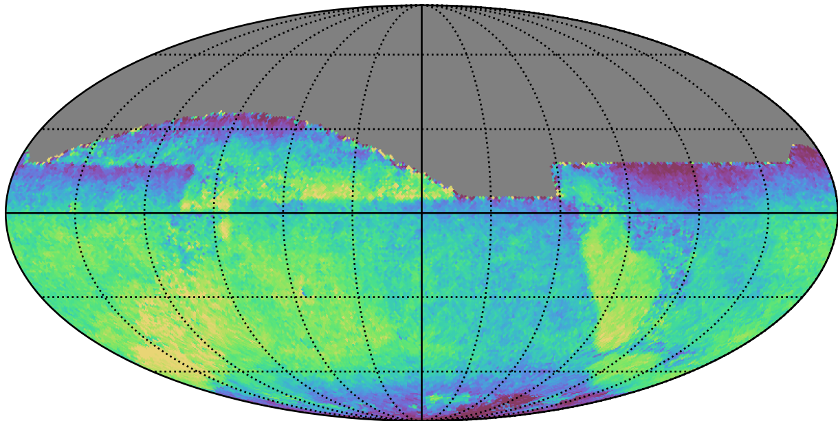
baseline_v3.0_10yrs All sky all bands: Median fiveSigmaDepth
