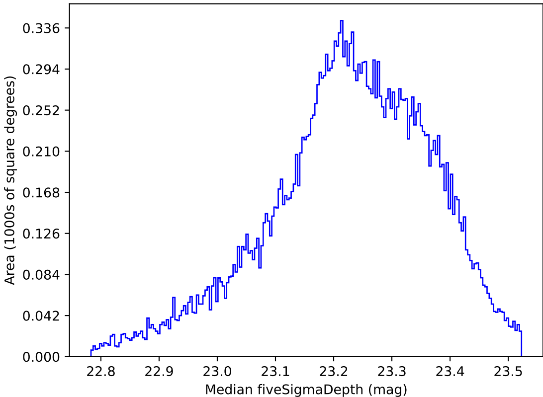
baseline_v3.0_10yrs All sky all bands: Median fiveSigmaDepth
