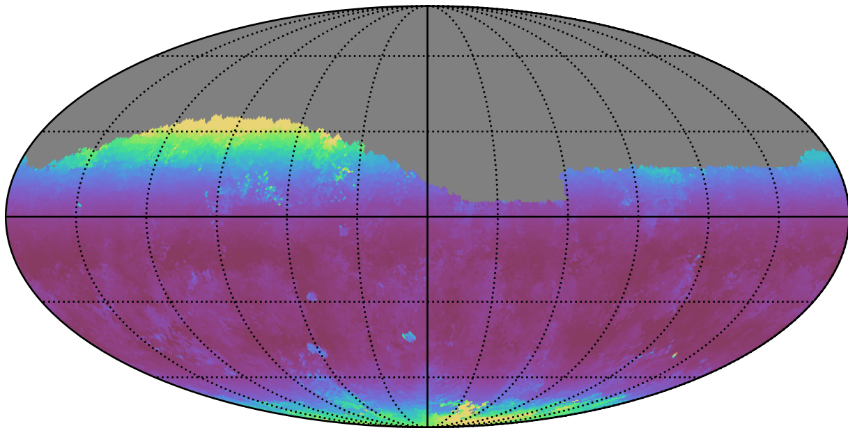
baseline_v3.0_10yrs Yr 1 z band: Median airmass
