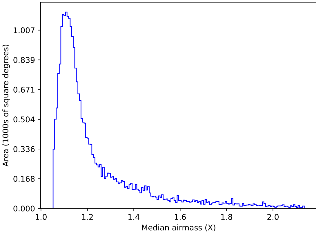
baseline_v3.0_10yrs Yr 1 z band: Median airmass
