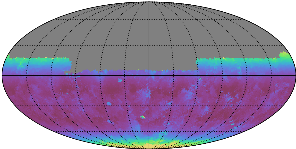
baseline_v3.0_10yrs Yr 1 y band: Median airmass
