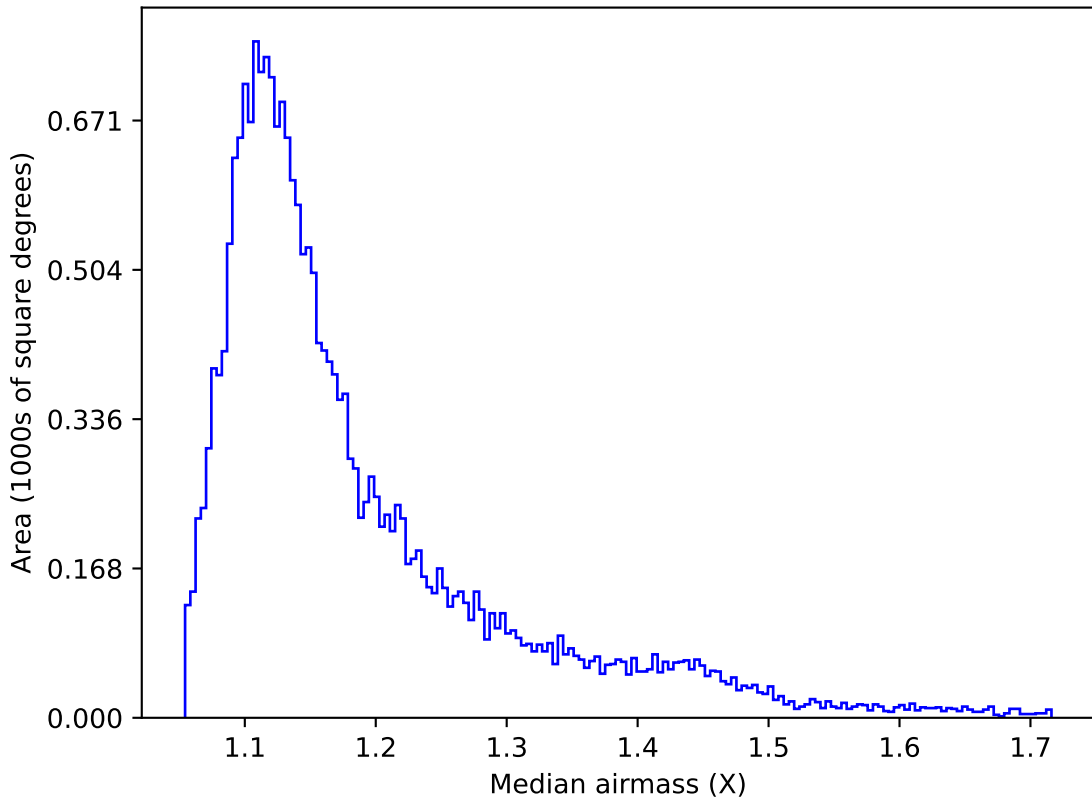
baseline_v3.0_10yrs Yr 1 y band: Median airmass
