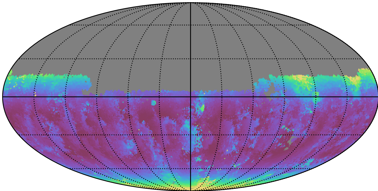
baseline_v3.0_10yrs Yr 1 u band: Median airmass
