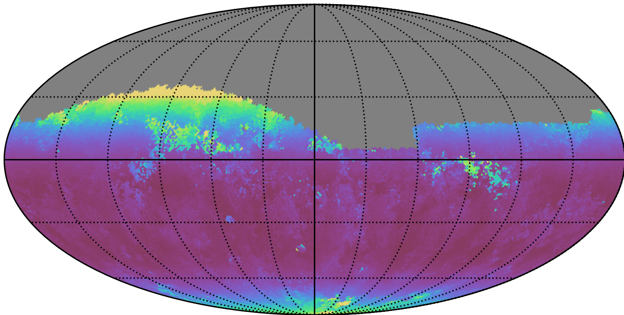
baseline_v3.0_10yrs Yr 1 r band: Median airmass
