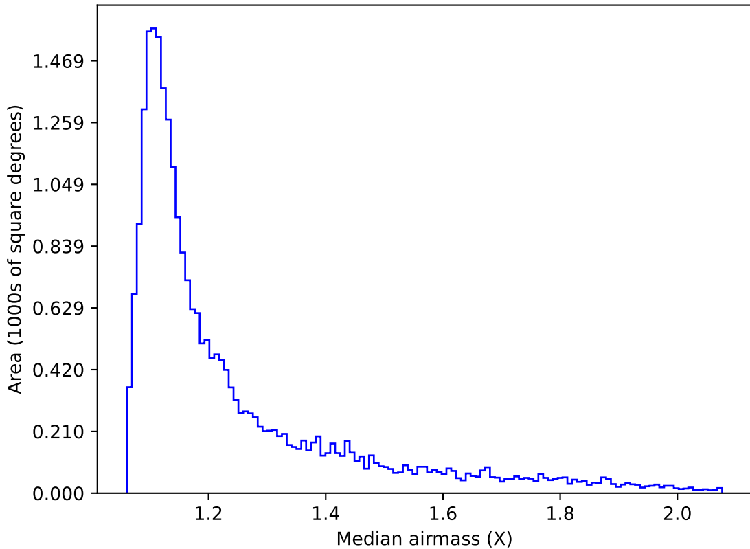
baseline_v3.0_10yrs Yr 1 r band: Median airmass
