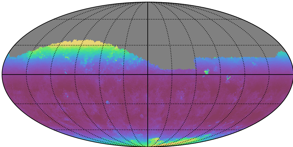
baseline_v3.0_10yrs Yr 1 i band: Median airmass
