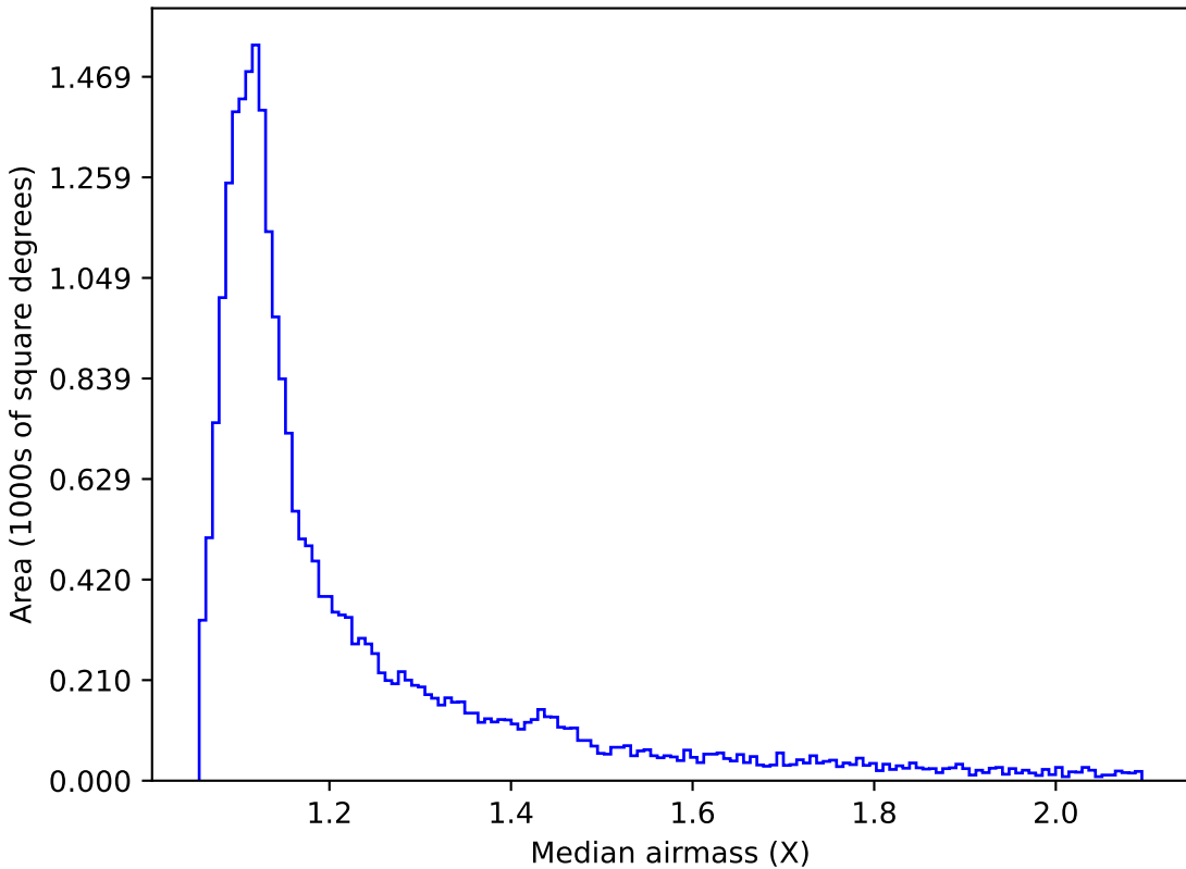
baseline_v3.0_10yrs Yr 1 i band: Median airmass
