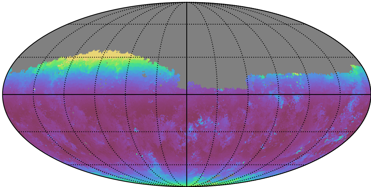
baseline_v3.0_10yrs Yr 1 g band: Median airmass
