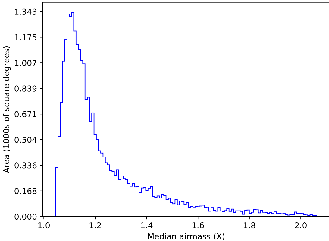
baseline_v3.0_10yrs Yr 1 g band: Median airmass
