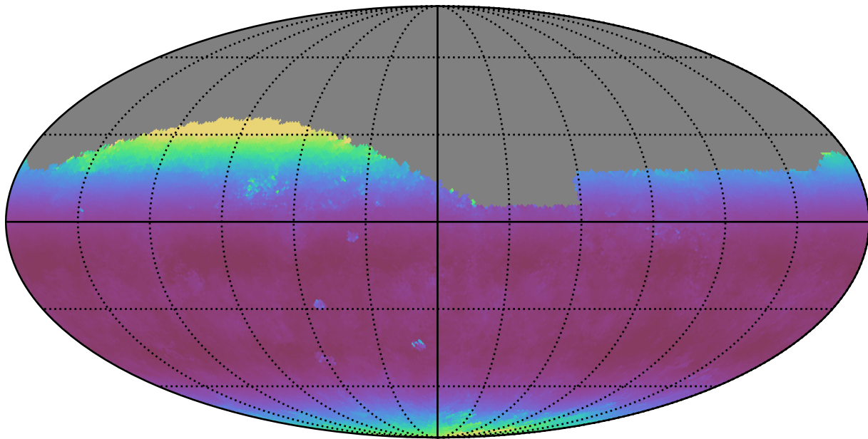
baseline_v3.0_10yrs Yr 1 all bands: Median airmass
