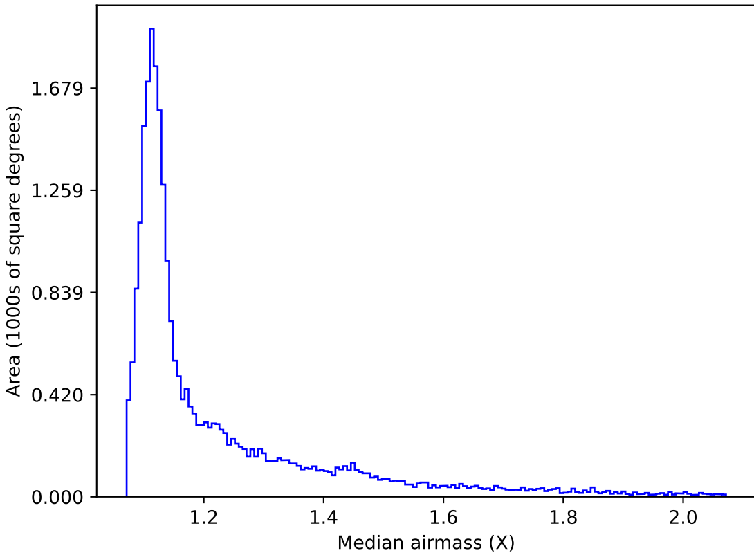
baseline_v3.0_10yrs Yr 1 all bands: Median airmass
