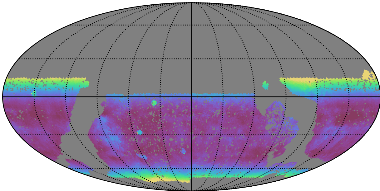
baseline_v3.0_10yrs WFD z band: Median airmass
