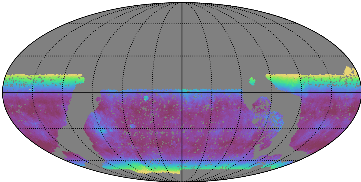
baseline_v3.0_10yrs WFD y band: Median airmass
