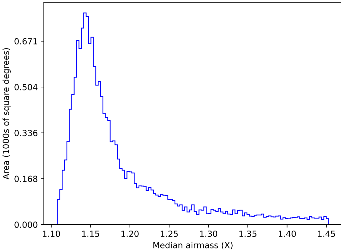
baseline_v3.0_10yrs WFD y band: Median airmass
