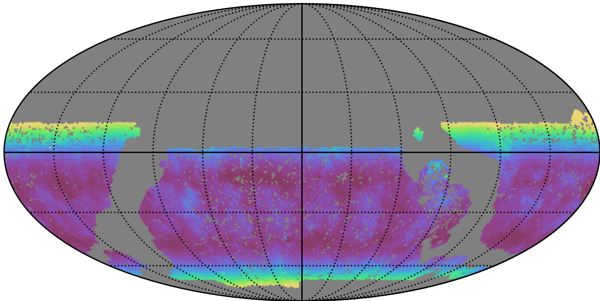
baseline_v3.0_10yrs WFD u band: Median airmass
