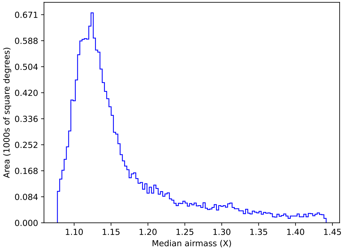
baseline_v3.0_10yrs WFD u band: Median airmass
