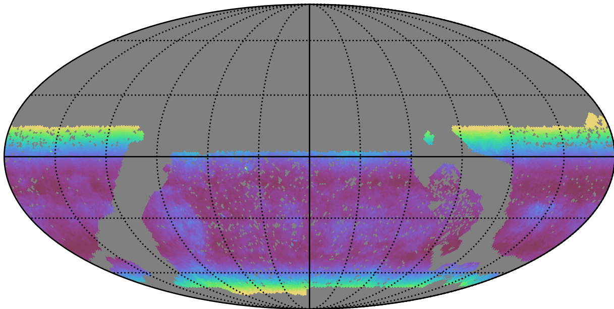
baseline_v3.0_10yrs WFD r band: Median airmass
