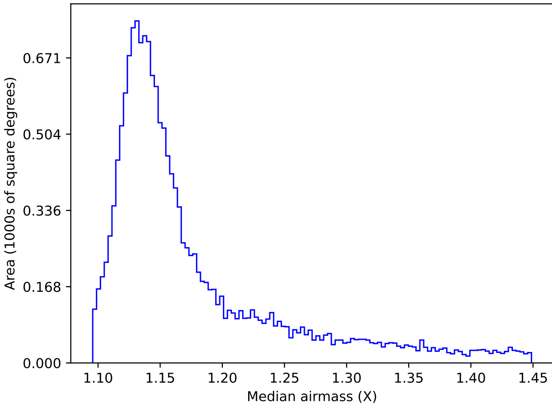
baseline_v3.0_10yrs WFD r band: Median airmass
