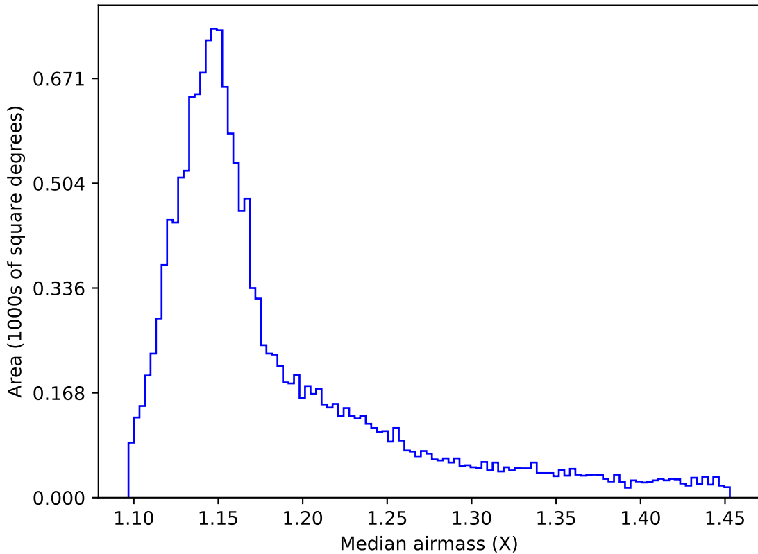
baseline_v3.0_10yrs WFD i band: Median airmass
