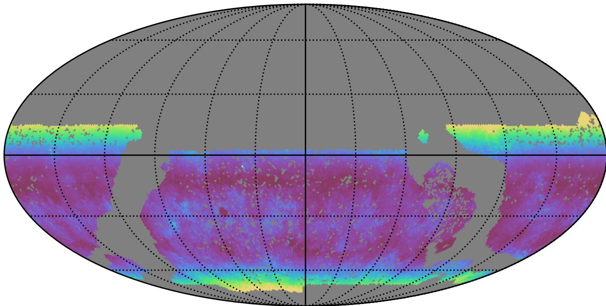
baseline_v3.0_10yrs WFD g band: Median airmass
