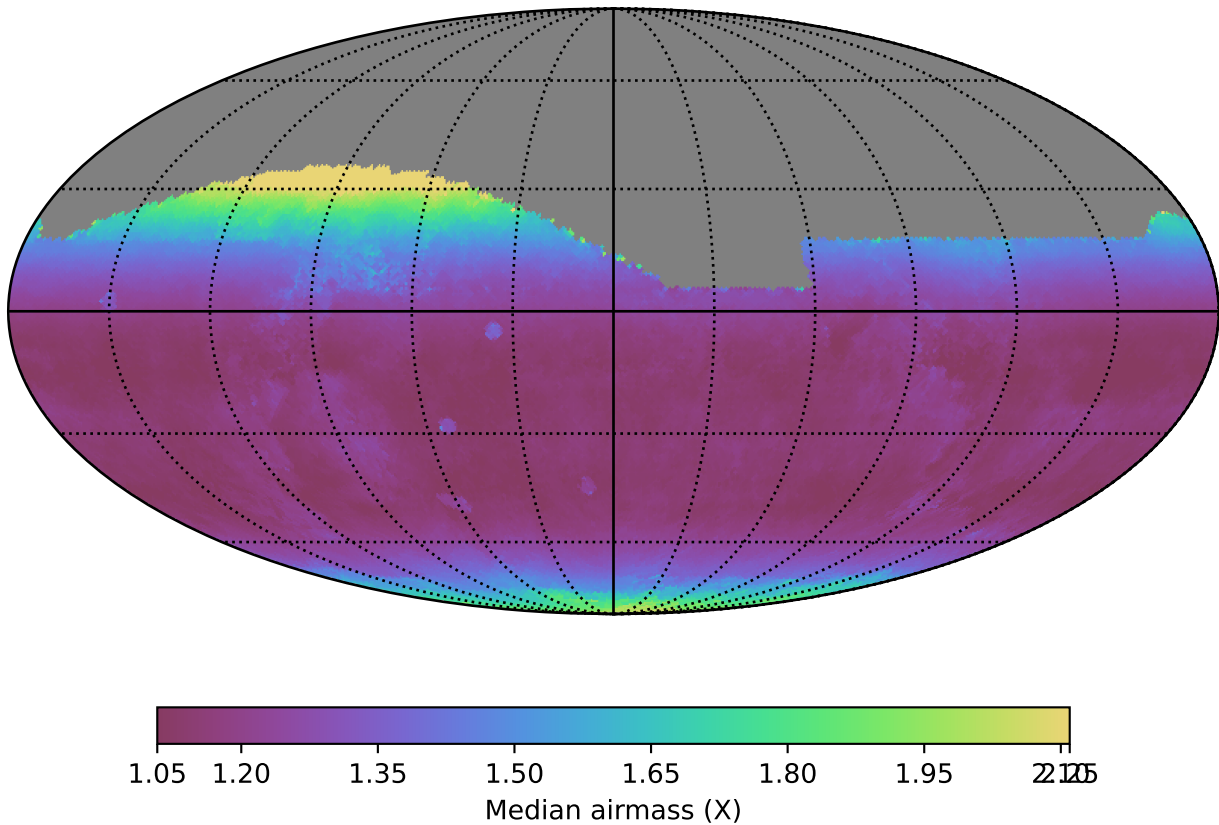
baseline_v3.0_10yrs All sky z band: Median airmass
