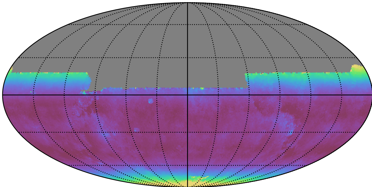
baseline_v3.0_10yrs All sky y band: Median airmass
