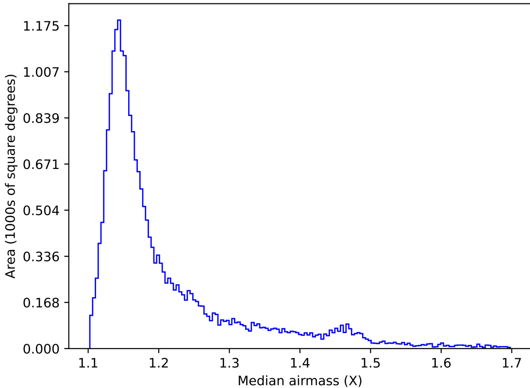
baseline_v3.0_10yrs All sky y band: Median airmass
