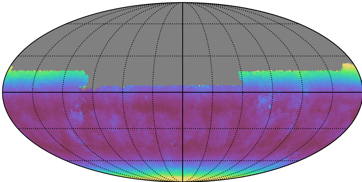
baseline_v3.0_10yrs All sky u band: Median airmass
