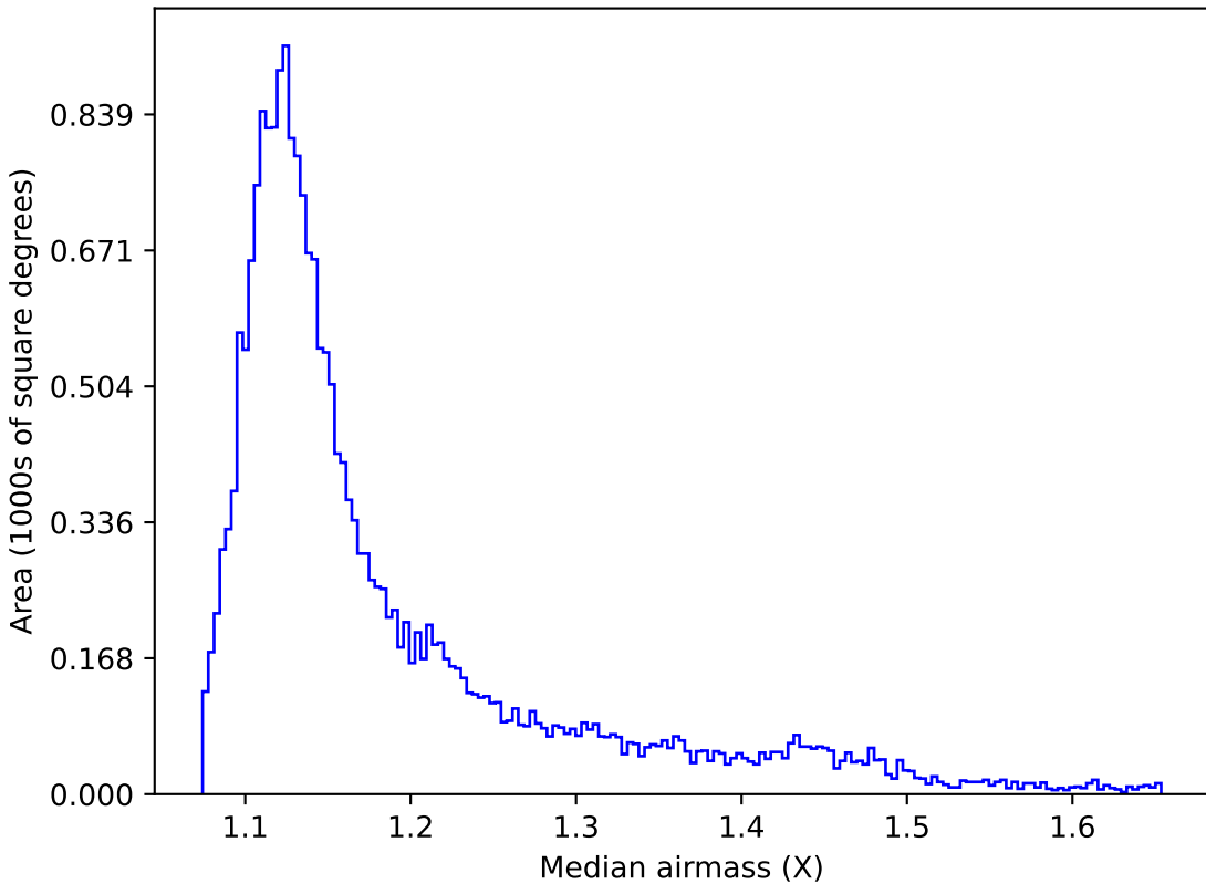
baseline_v3.0_10yrs All sky u band: Median airmass
