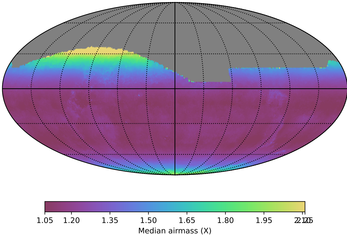
baseline_v3.0_10yrs All sky r band: Median airmass
