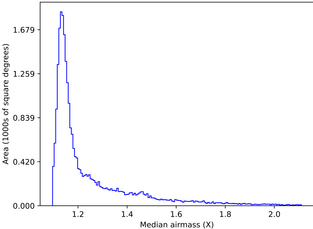
baseline_v3.0_10yrs All sky r band: Median airmass
