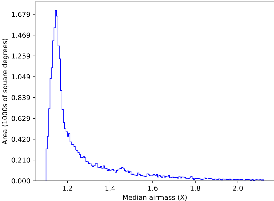
baseline_v3.0_10yrs All sky i band: Median airmass
