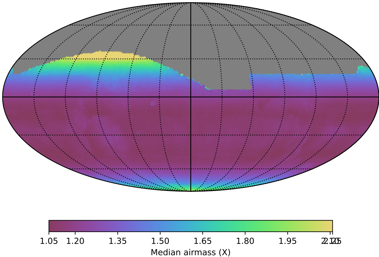
baseline_v3.0_10yrs All sky all bands: Median airmass
