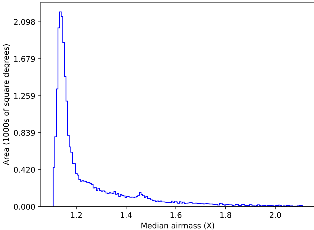
baseline_v3.0_10yrs All sky all bands: Median airmass
