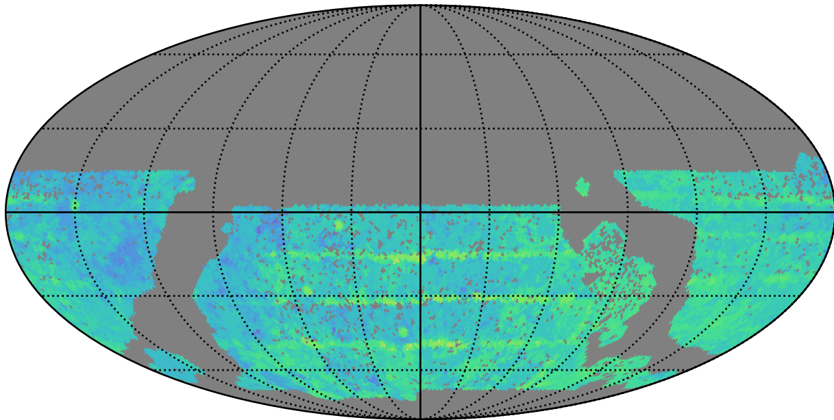
baseline_v3.0_10yrs WFD z band: Median Season Length
