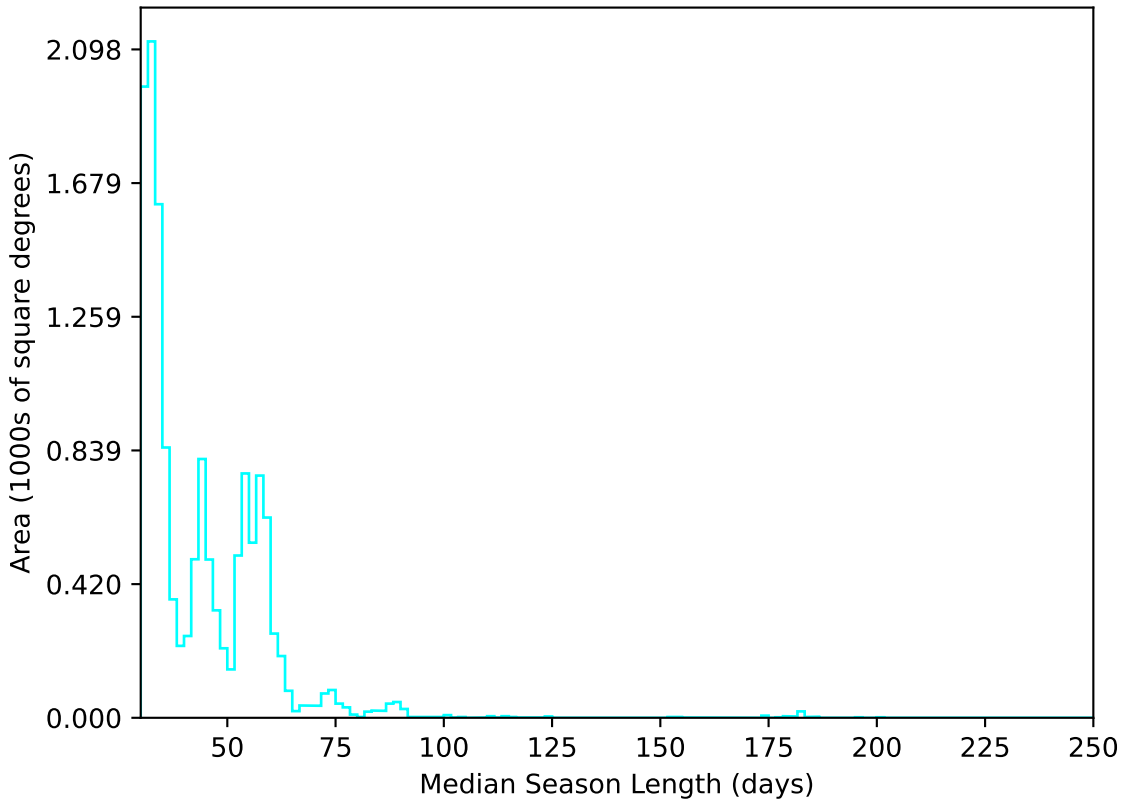
baseline_v3.0_10yrs WFD u band: Median Season Length
