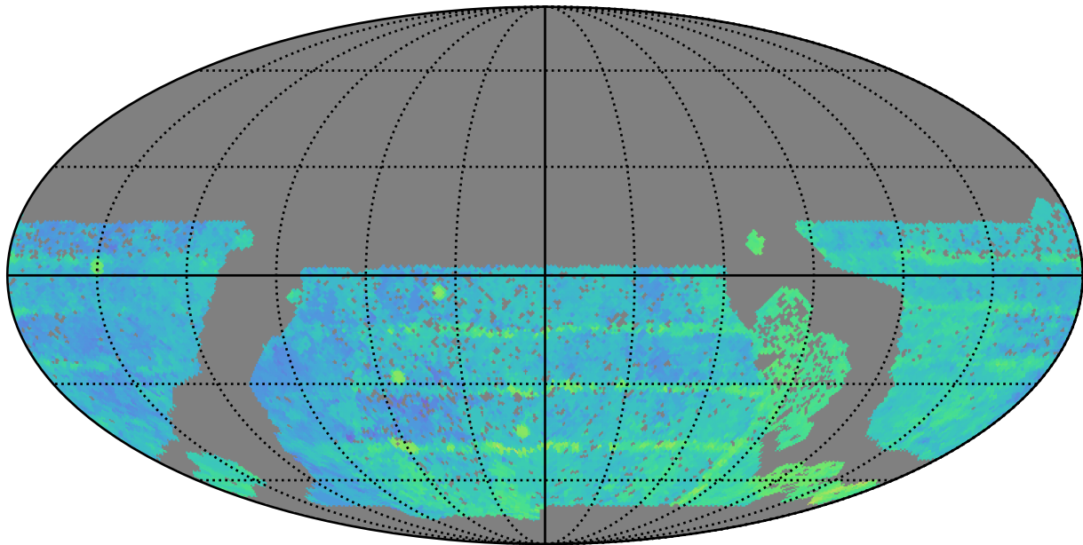
baseline_v3.0_10yrs WFD r band: Median Season Length
