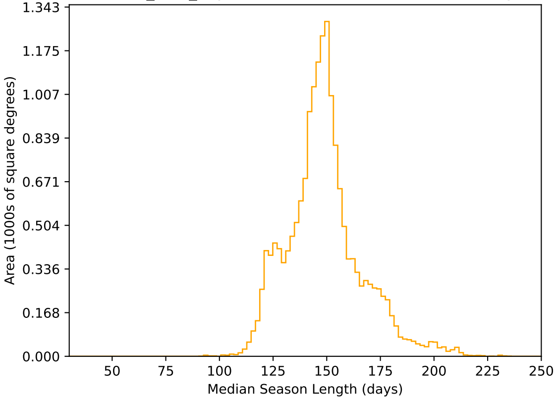
baseline_v3.0_10yrs WFD r band: Median Season Length
