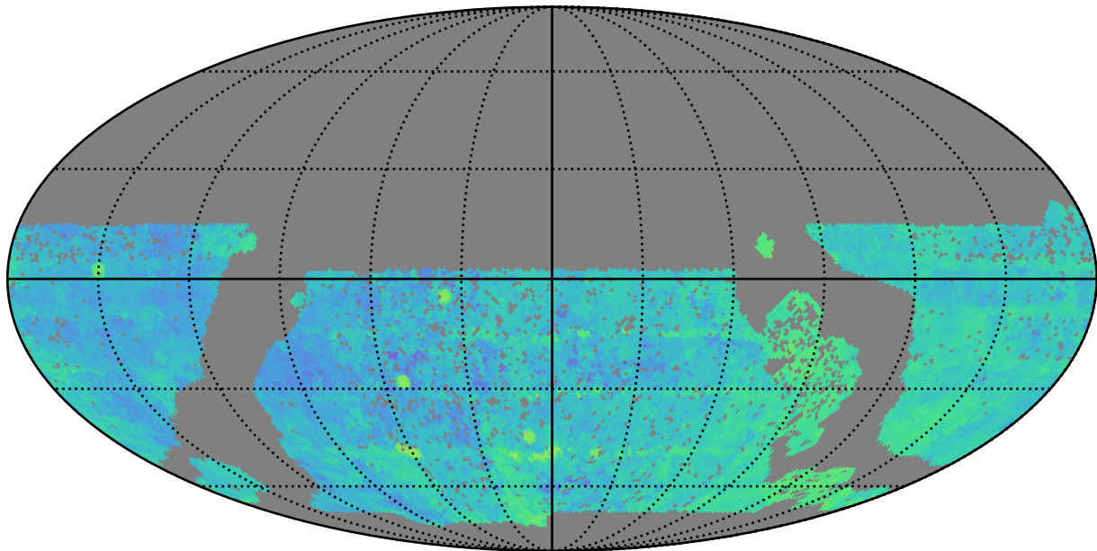
baseline_v3.0_10yrs WFD i band: Median Season Length
