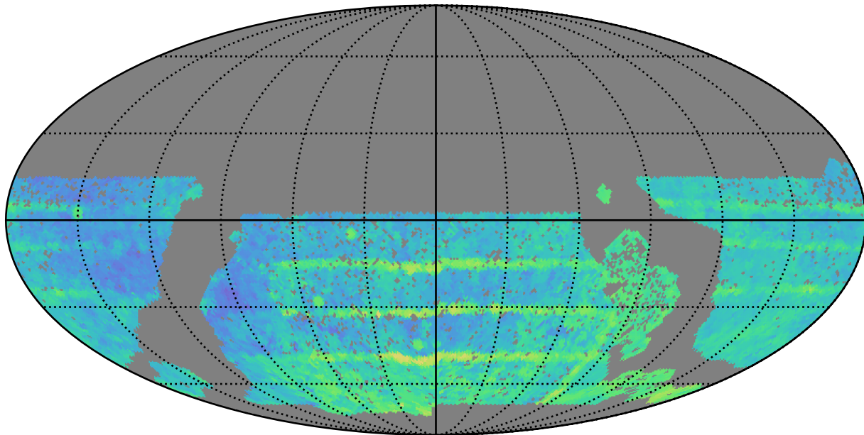
baseline_v3.0_10yrs WFD all bands: Median Season Length
