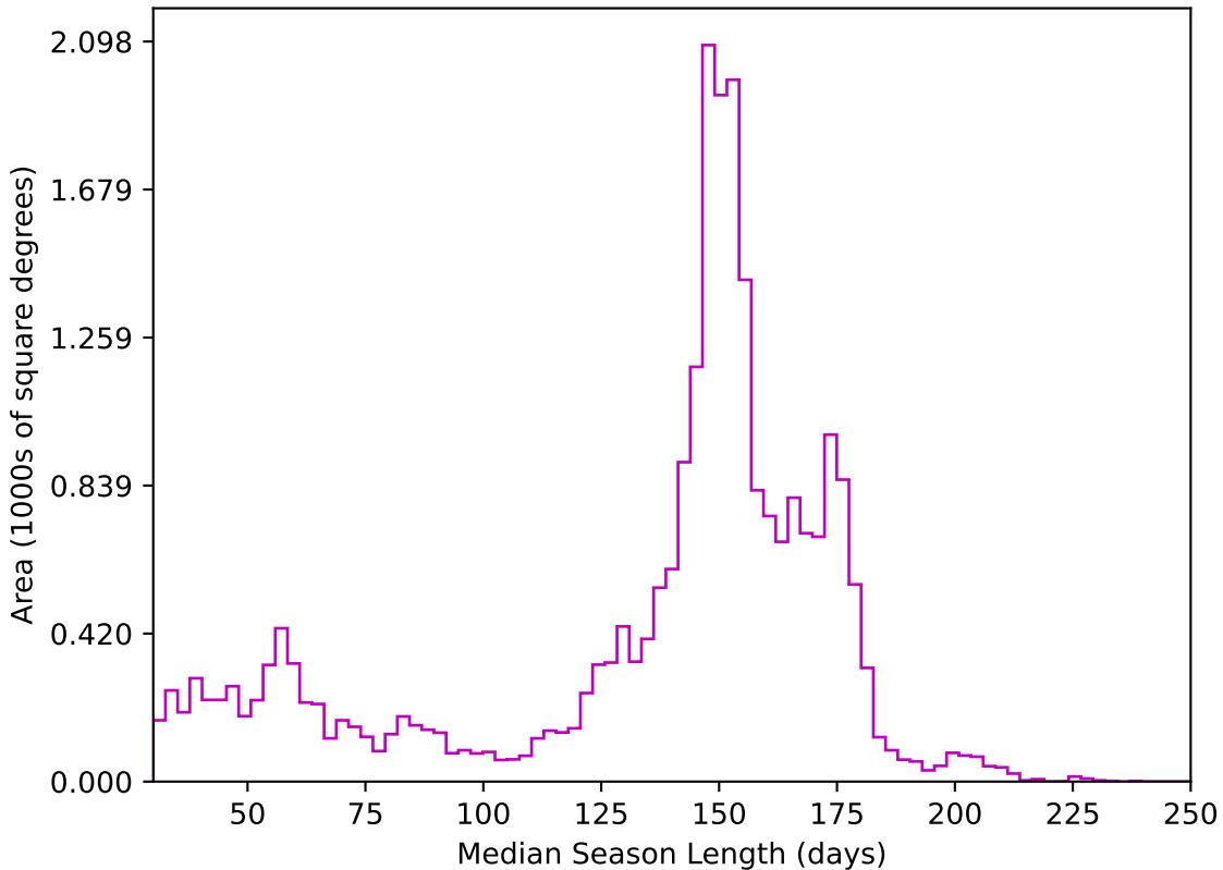
baseline_v3.0_10yrs All sky z band: Median Season Length
