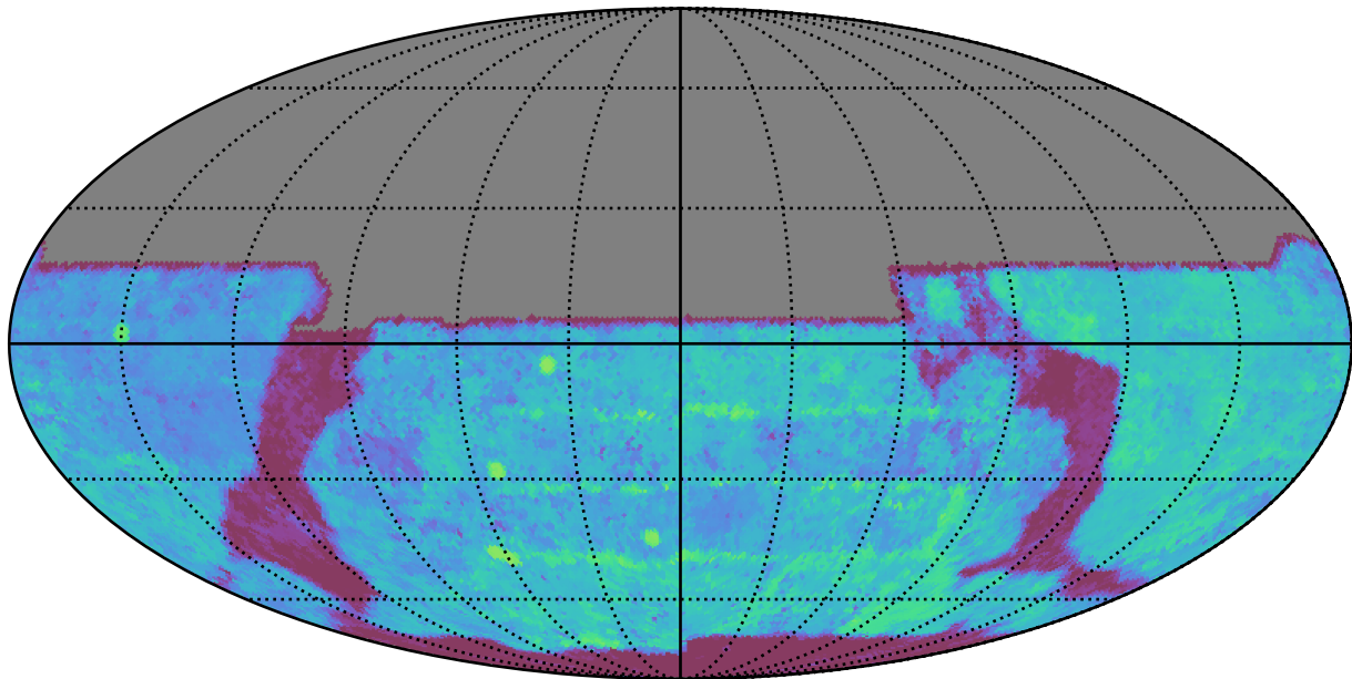
baseline_v3.0_10yrs All sky y band: Median Season Length
