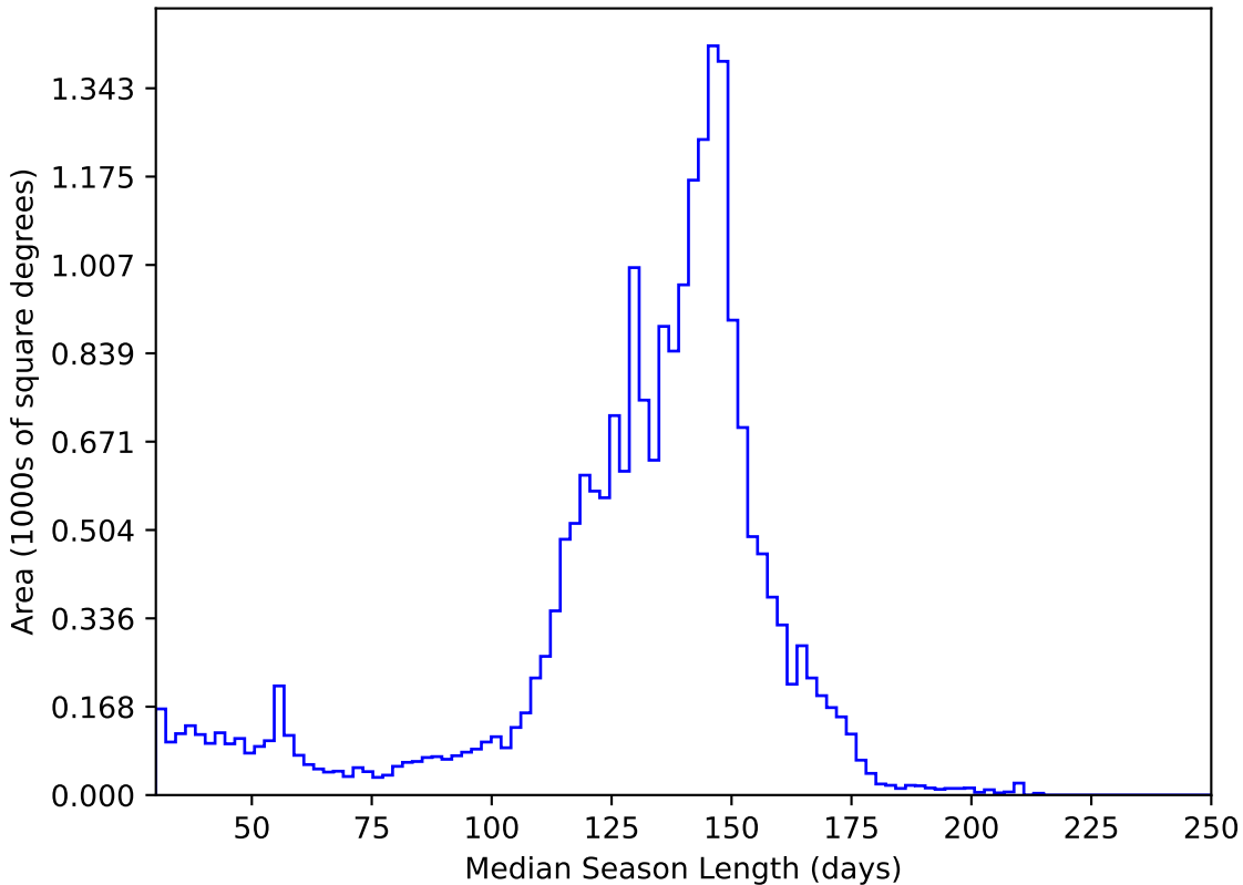
baseline_v3.0_10yrs All sky y band: Median Season Length
