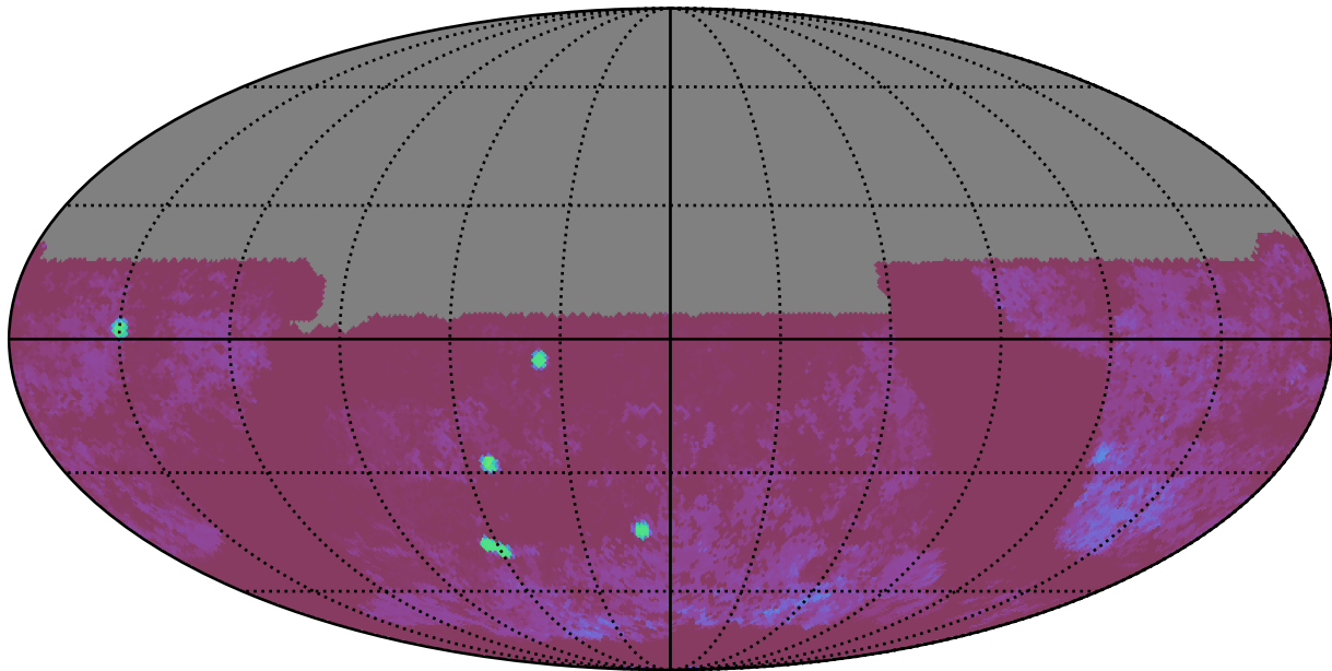
baseline_v3.0_10yrs All sky u band: Median Season Length
