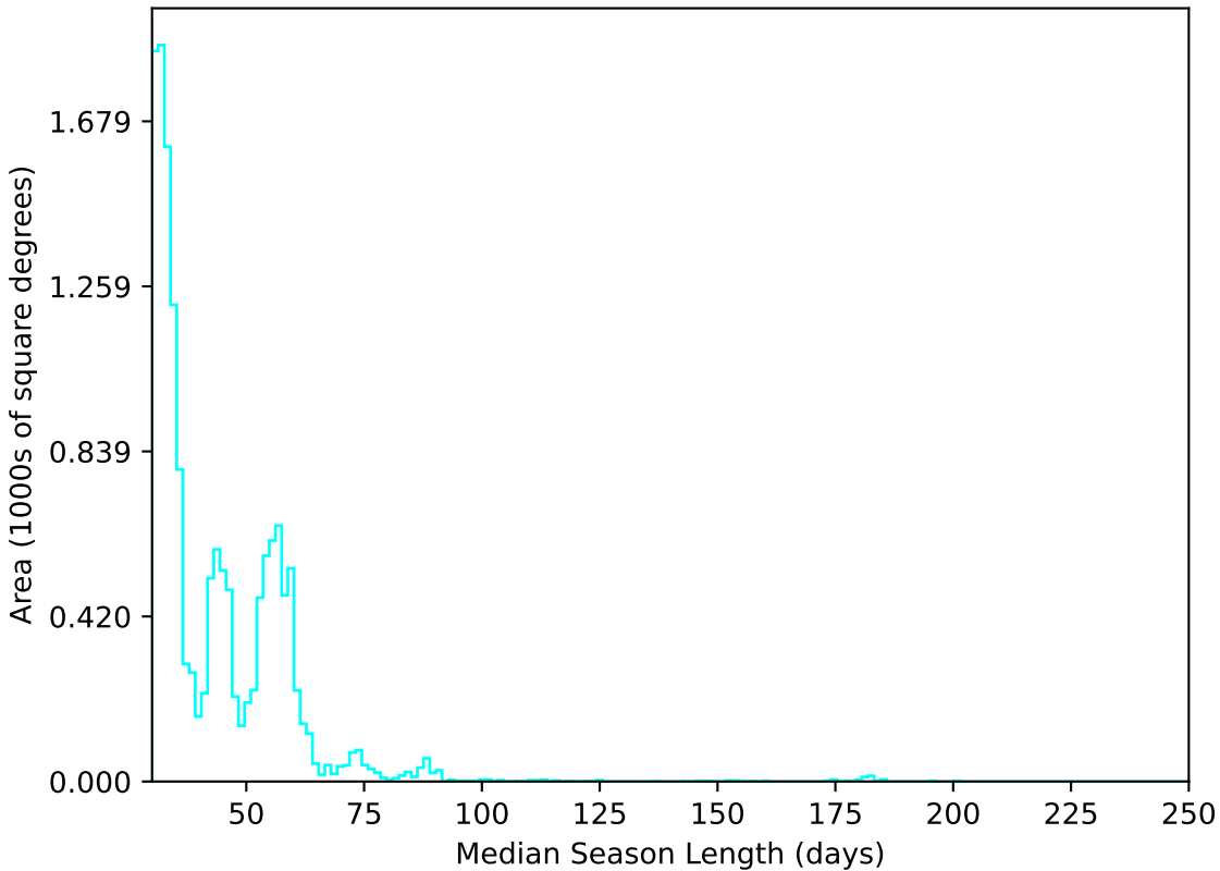
baseline_v3.0_10yrs All sky u band: Median Season Length
