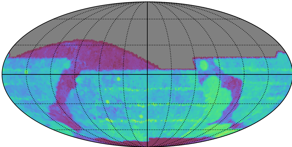
baseline_v3.0_10yrs All sky r band: Median Season Length
